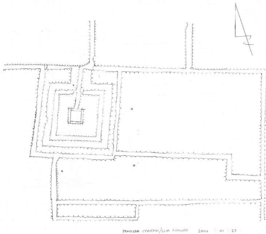
A map of Itabuki Palace Site, drawn with plane table survey method by participants (24-25 January)
