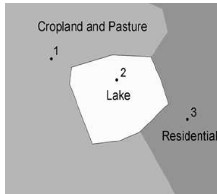
Vector data
