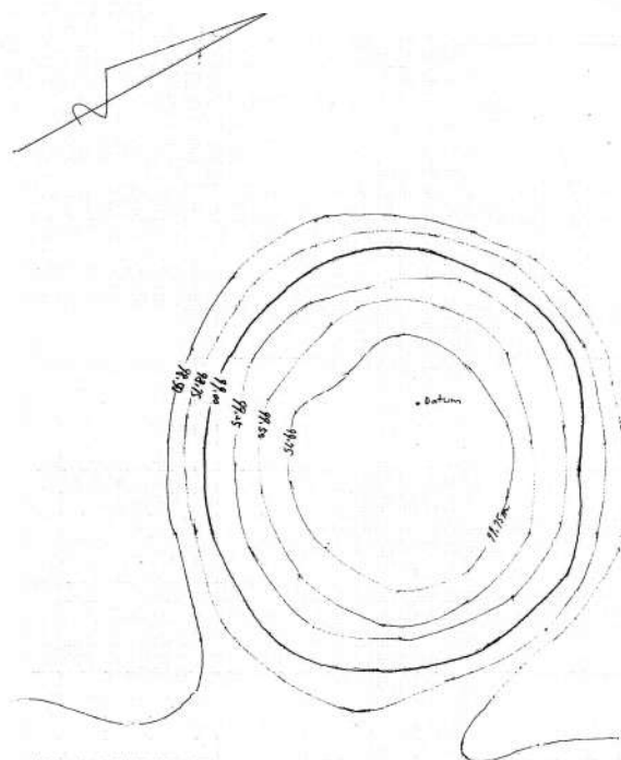
A map of Itabuki Palace Site, drawn with plane table survey method by participants (24-25 January)
