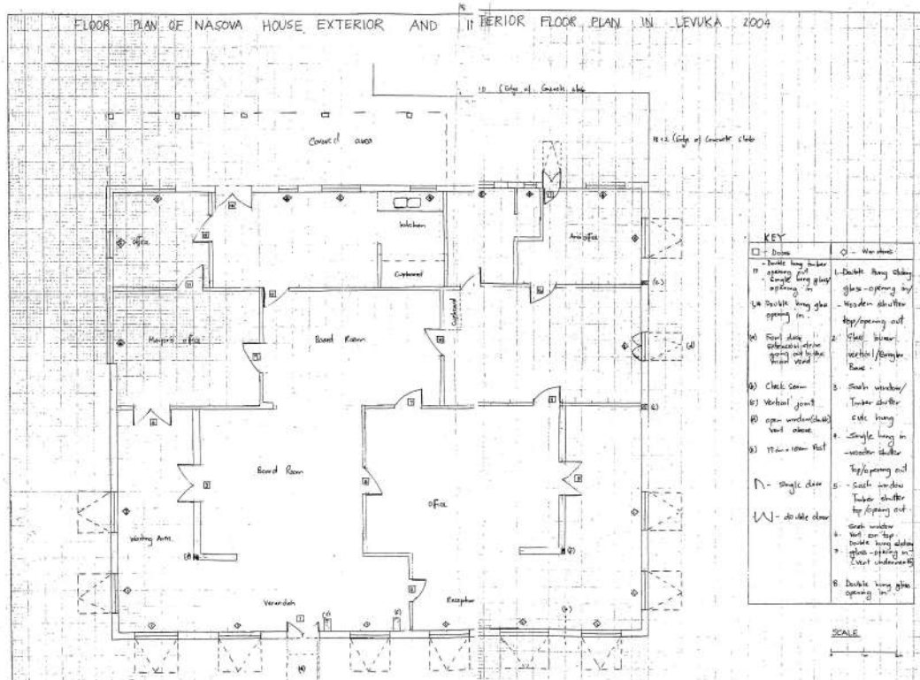
Fig.1 Hand drawn map of Nasova Final drawing was drawn up by hand using ruler and protector
