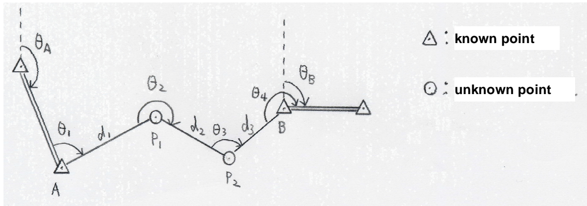
Connected traverse
