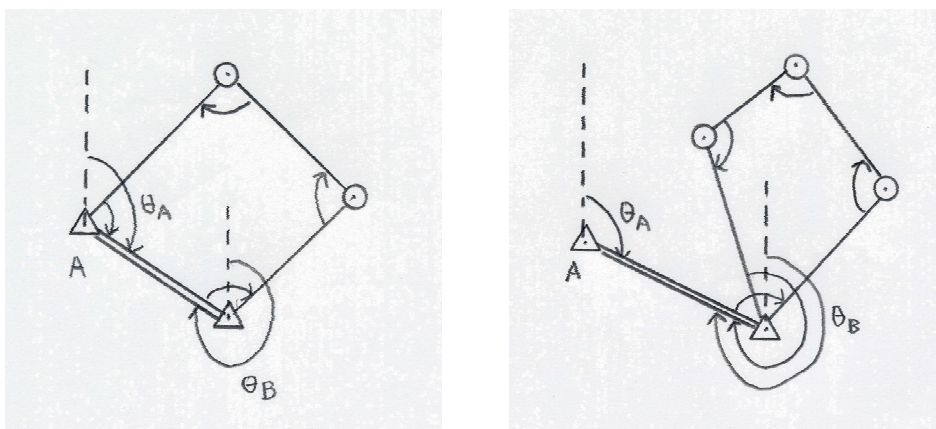
Closed traverse
