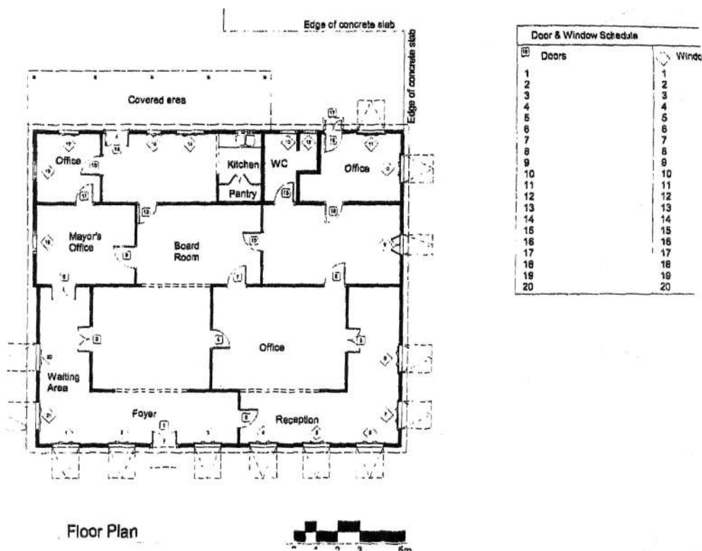
Fig.2 Auto CAD Drawing Also drawn up one participant who was familiar with Auto CAD software
